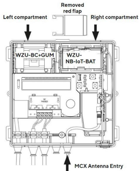
Figure 4: Mounting instructions
