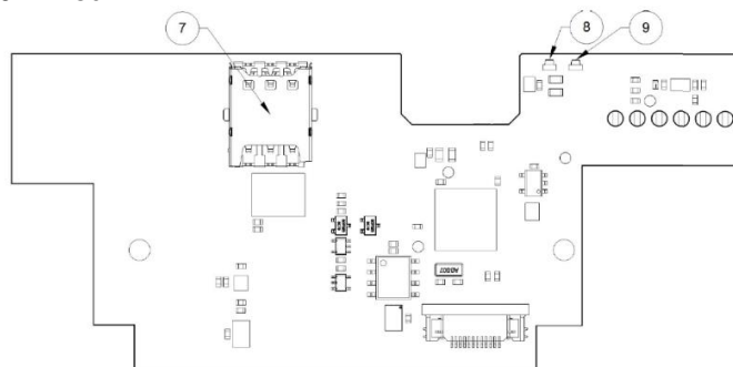
Figure 2: CMi6110 backside
