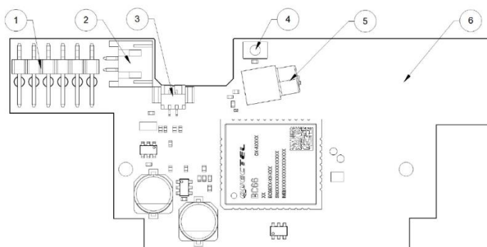
Figure 1: CMi6110 frontside
